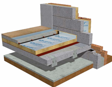
Suspended beam and block floor
