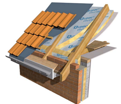
Pitched roof: QR between & below rafters
